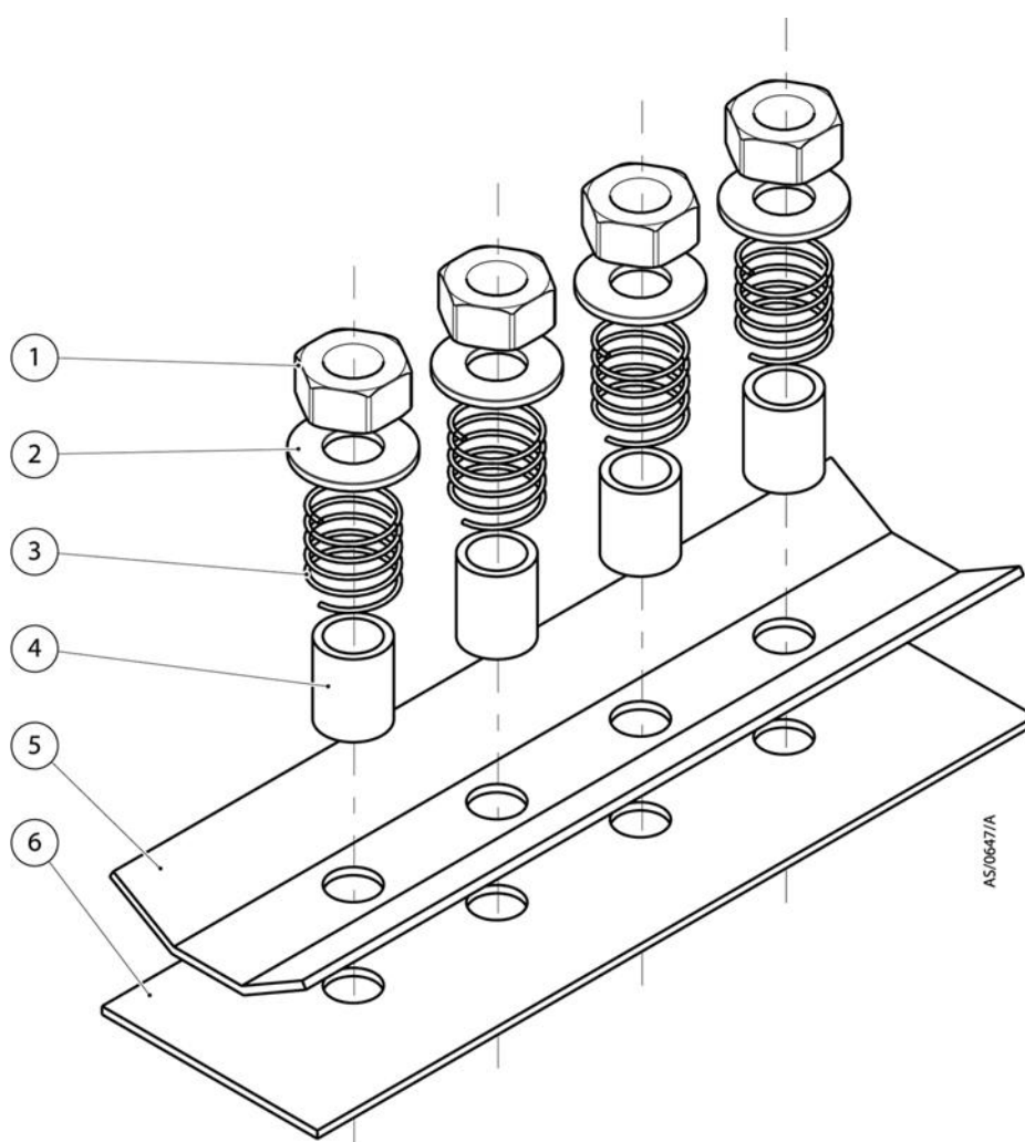
Figure 1 - E2M275 Spring loaded exhaust valve assembly
